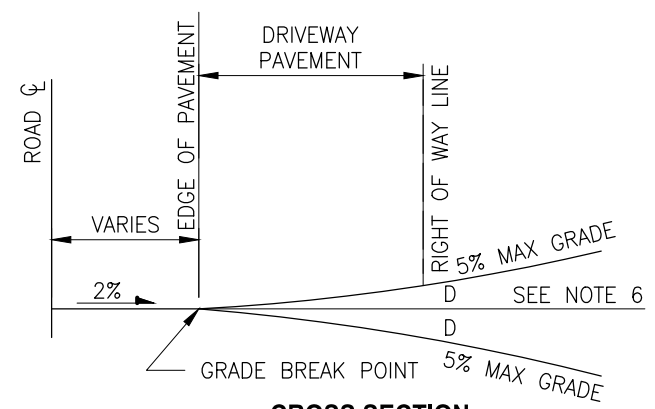
CROSS SECTION
