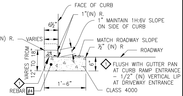
DEPRESSED CURB SECTION
